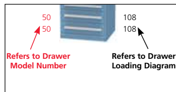
XSEP1405AL 4 Drawers 68 Compartments Usable Drawer Heights 2-1/4 in (57 mm) 3-7/8 in (98 mm) 4-5/8 in (117 mm) 10-1/8 in (257 mm) 246 lbs (111 kg) Shipping Weight
