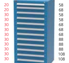
XSEP3047AL 12 Drawers 224 Compartments 628 lbs. (285 kg.) Shipping Weight
