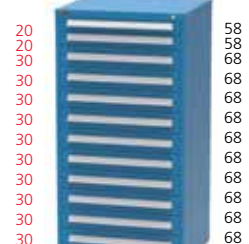
XSCU3047AL 12 Drawers 248 Compartments 626 lbs. (284 kg.) Shipping Weight
